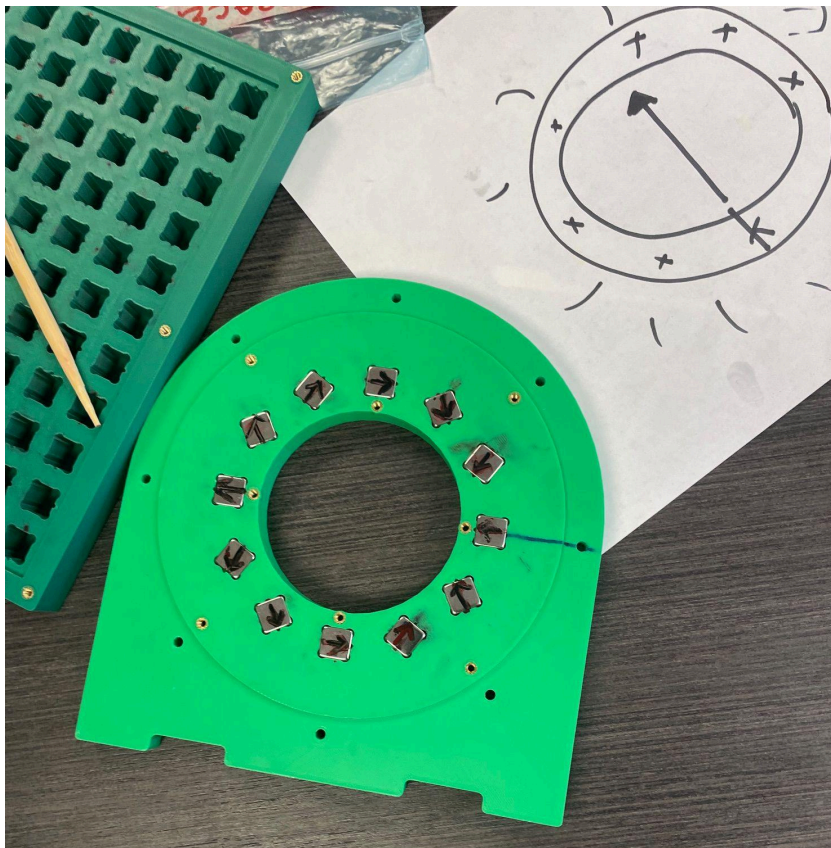
Example of Ring 42 after putting magnets.
